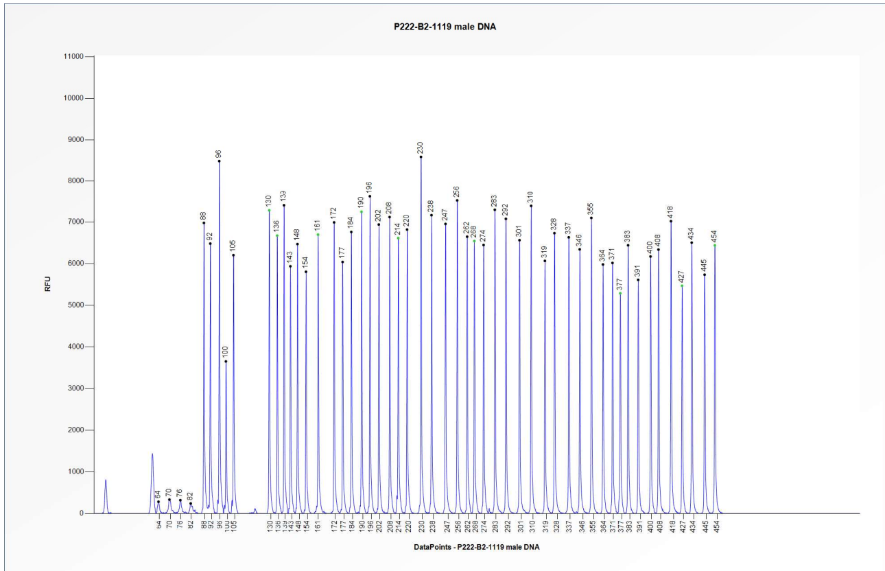
Figure 1. Capillary electrophoresis pattern from a sample of approximately 50 ng human male control DNA analysed with SALSA MLPA Probemix P222 LCA mix-2 (B2-1119).
