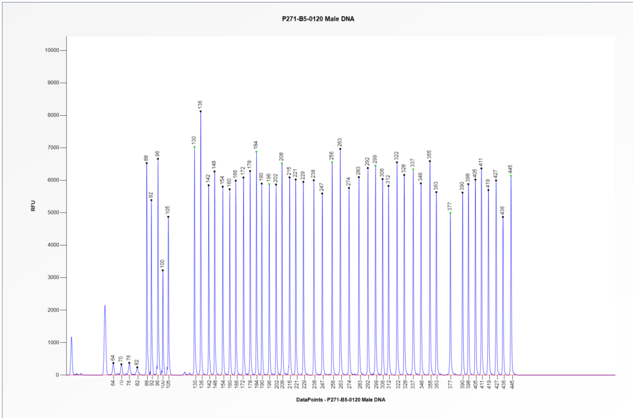
Figure 1. Capillary electrophoresis pattern from a sample of approximately 50 ng human male control DNA analysed with SALSA MLPA Probemix P271 COL1A1 (B5-0120).
