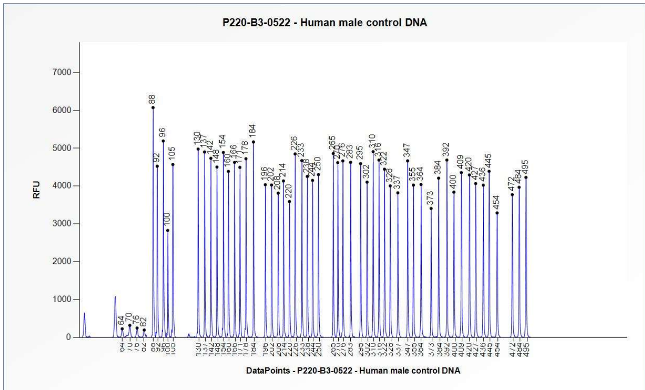
Figure 1. Capillary electrophoresis pattern from a sample of approximately 50 ng human male control DNA analysed with SALSA MLPA Probemix P220 Obesity (B3-0522).
