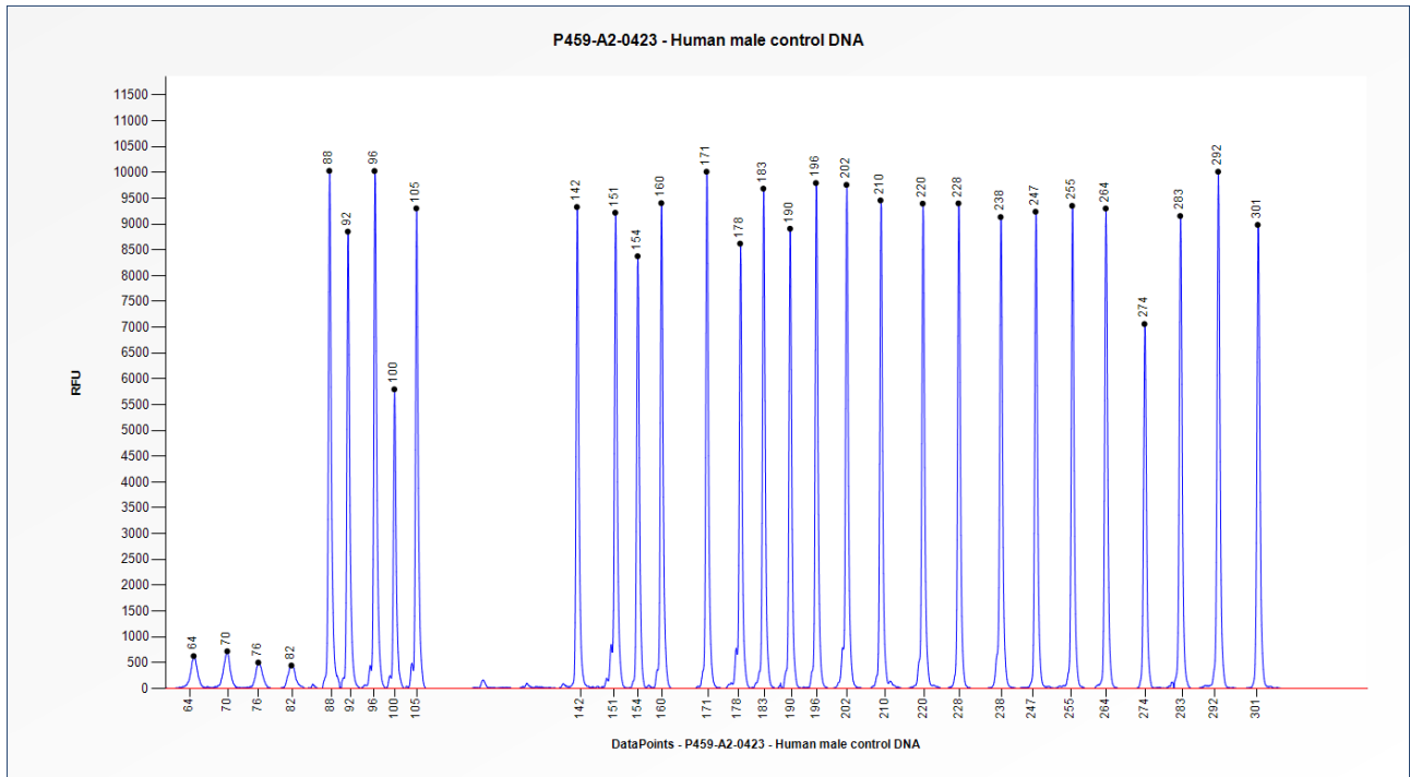
Figure 1. Capillary electrophoresis pattern from a sample of approximately 50 ng human male control DNA analysed with SALSA MLPA Probemix P459 SERPINA1 (A2-0423).
