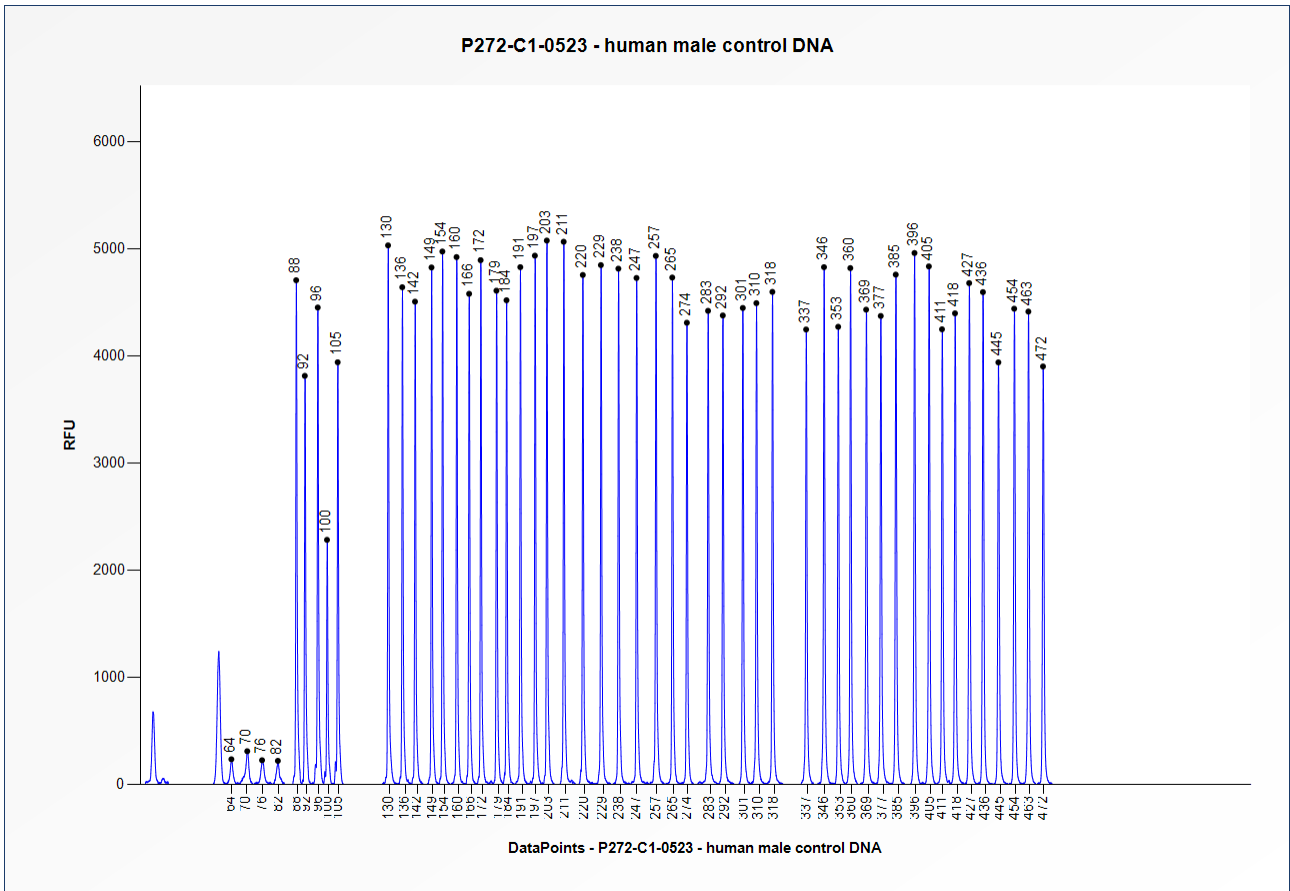
Figure 1. Capillary electrophoresis pattern from a sample of approximately 50 ng human male control DNA analysed with SALSA MLPA Probemix P272 COL1A2 (C1-0523).
