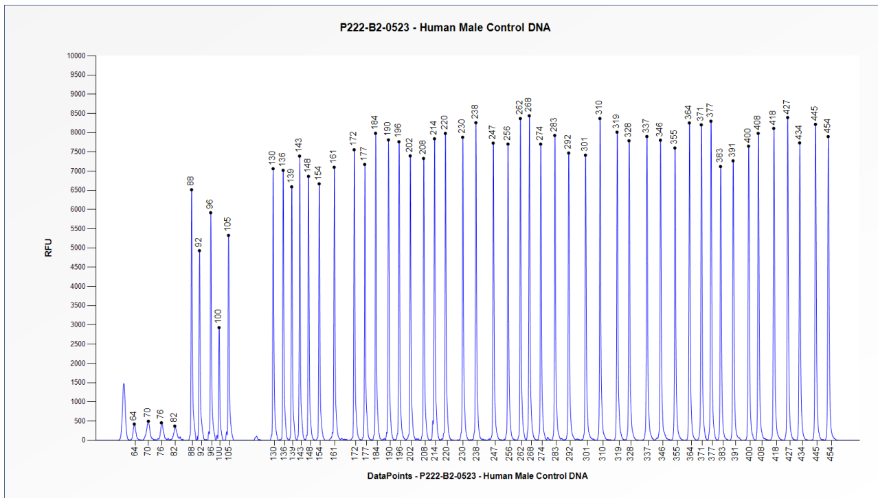
Figure 1. Capillary electrophoresis pattern from a sample of approximately 50 ng human male control DNA analysed with SALSA MLPA Probemix P222 LCA mix-2 (B2-0523).
