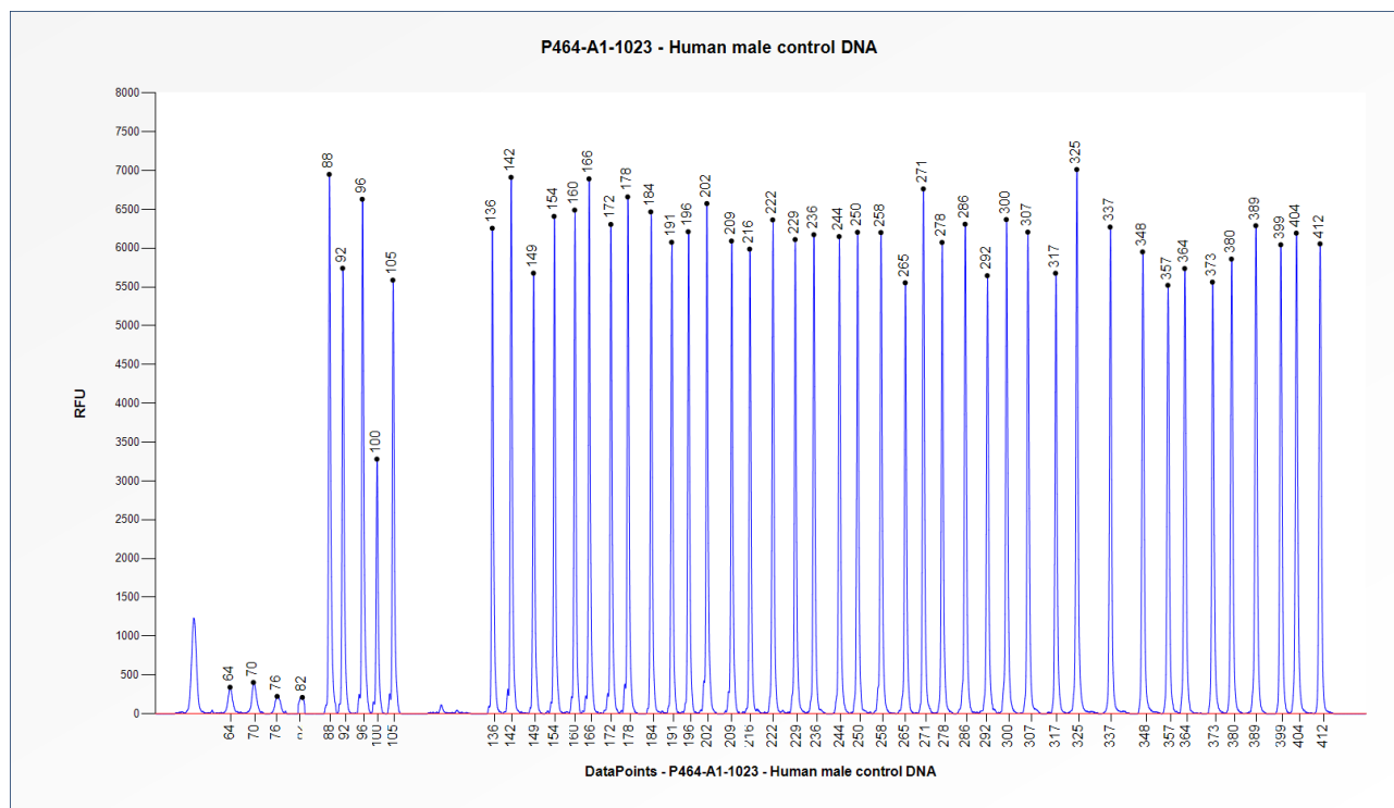
Figure 1. Capillary electrophoresis pattern from a sample of approximately 50 ng human male control DNA analysed with SALSA MLPA Probemix P464 INSR (A1-1023).
