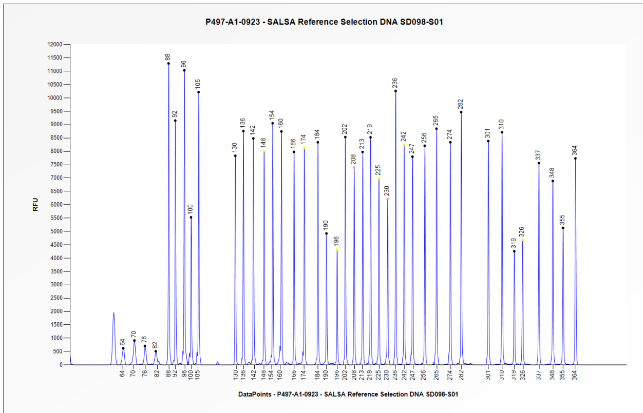
Figure 1. Capillary electrophoresis pattern from SALSA Reference Selection DNA SD098-S01 (approximately 50 ng) analysed with SALSA MLPA Probemix P497 Opsin (A1-0923).
