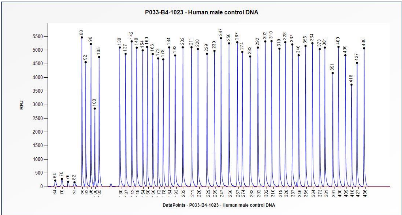
Figure 1. Capillary electrophoresis pattern from a sample of approximately 50 ng human male control DNA analysed with SALSA MLPA Probemix P033 CMT1 (B4-1023).
