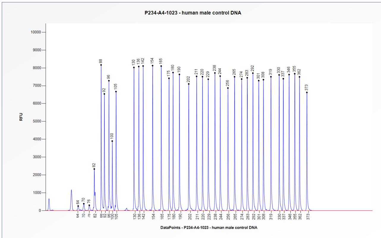
Figure 1. Capillary electrophoresis pattern from a sample of approximately 50 ng human male control DNA analysed with SALSA MLPA Probemix P234 GATA3 – GATA4 (A4-1023).
