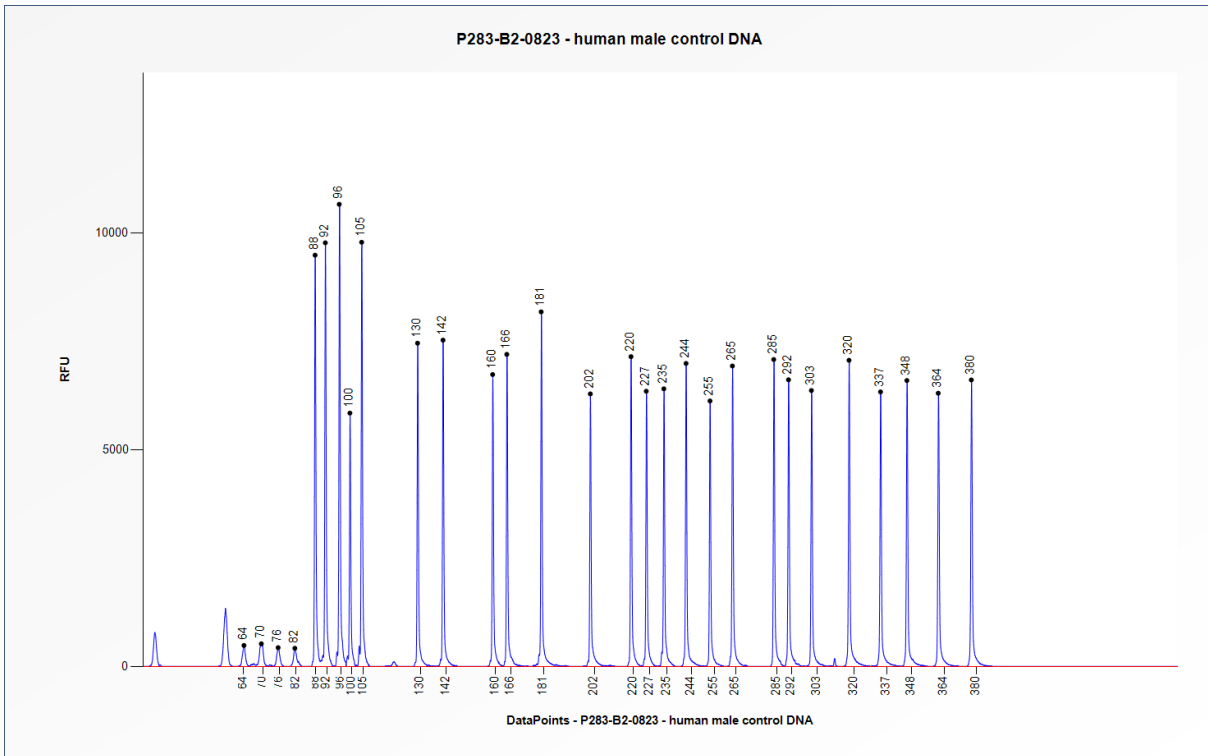
Figure 1. Capillary electrophoresis pattern from a sample of approximately 50 ng human male control DNA analysed with SALSA MLPA Probemix P283 TPMT (B2-0823).
