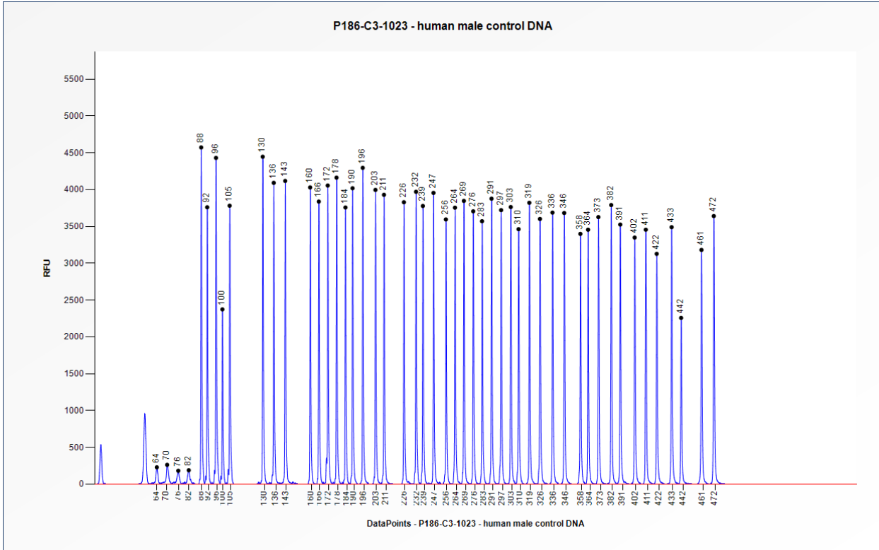
Figure 1. Capillary electrophoresis pattern from a sample of approximately 50 ng human male control DNA analysed with SALSA MLPA Probemix P186 PAX3 MITF SOX10 (C3-1023).
