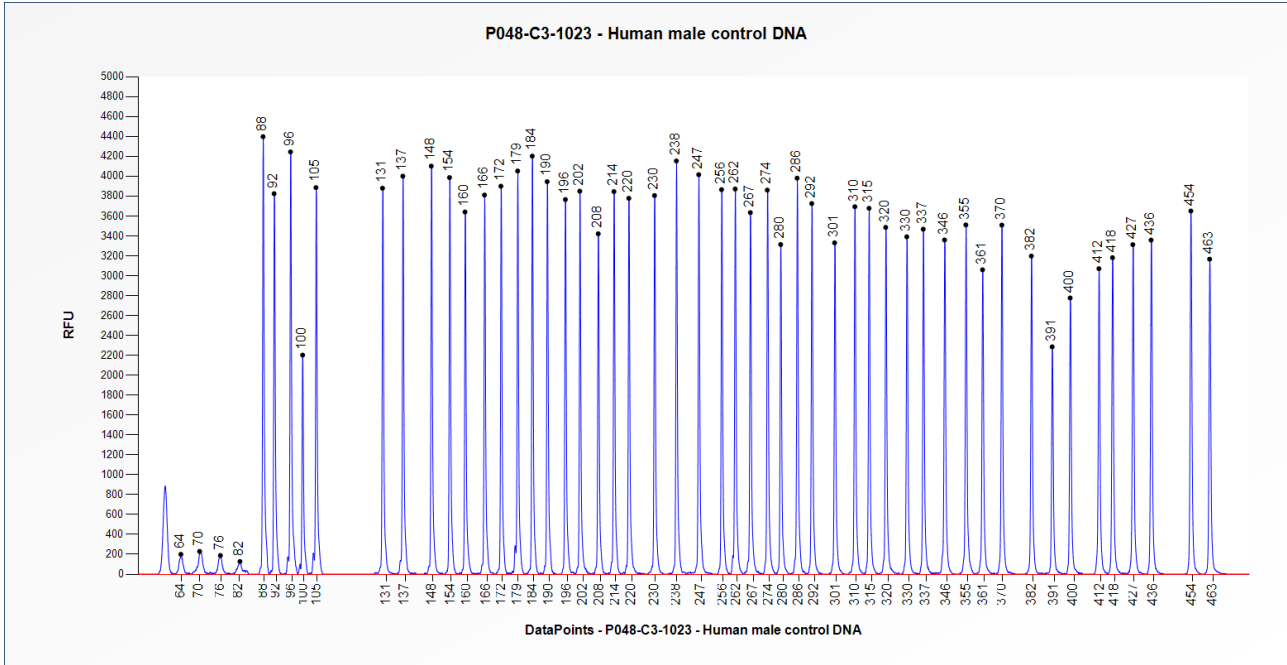
Figure 1. Capillary electrophoresis pattern from a sample of approximately 50 ng human male control DNA analysed with SALSA MLPA Probemix P048 LMNA/MYOT/ZMPSTE24 (C3-1023).
