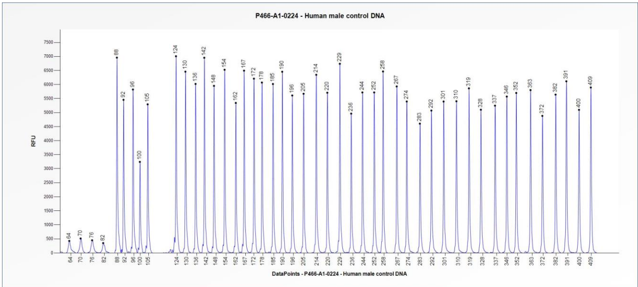
Figure 1. Capillary electrophoresis pattern from a sample of approximately 50 ng human male control DNA analysed with SALSA MLPA Probemix P466 CDC73 (A1-0224).
