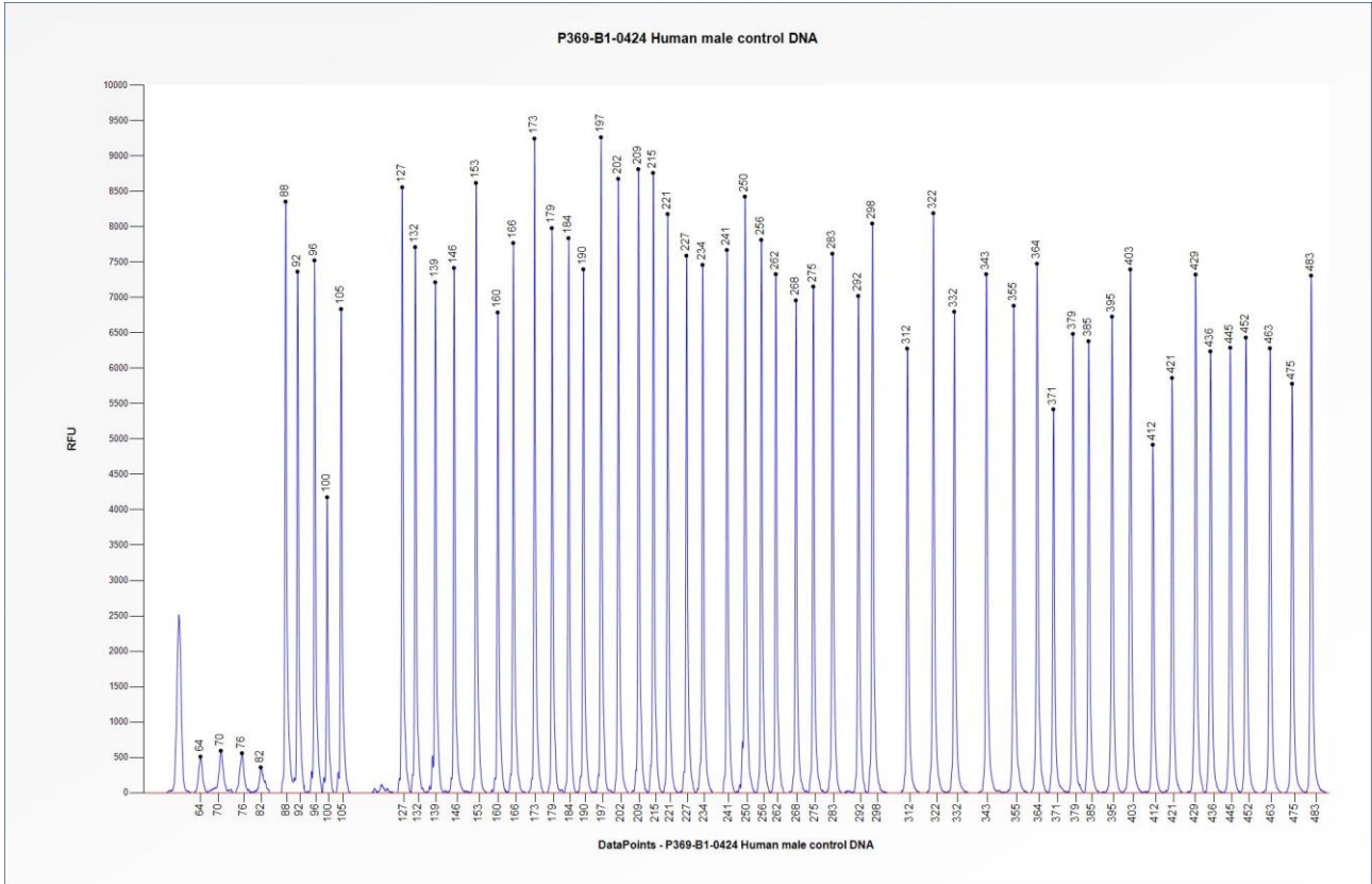
Figure 1. Capillary electrophoresis pattern from a sample of approximately 50 ng human male control DNA analysed with SALSA MLPA Probemix P369 Smith Magenis (B1-0424).
