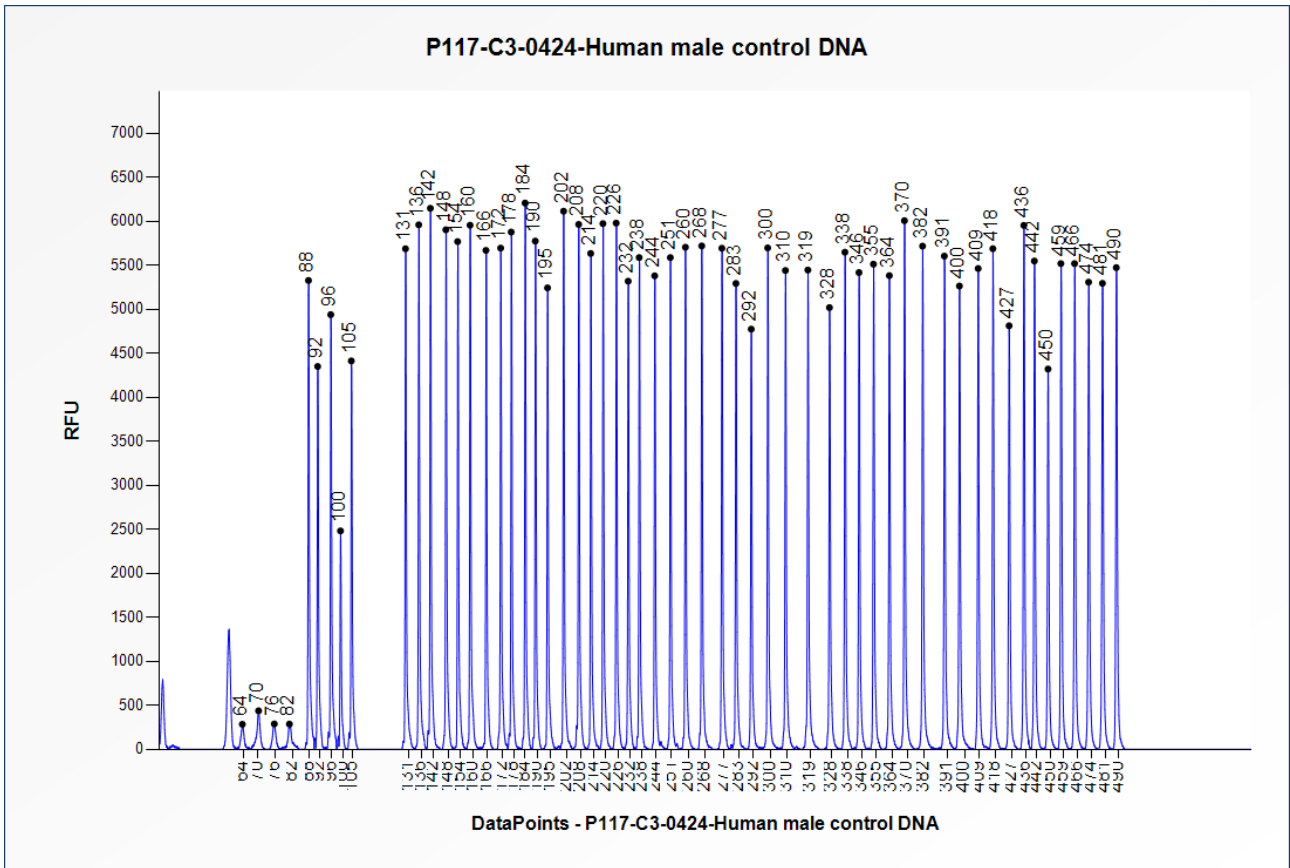
Figure 1. Capillary electrophoresis pattern from a sample of approximately 50 ng human male control DNA analysed with SALSA MLPA Probemix P117 ABCC8 (C3-0424).
