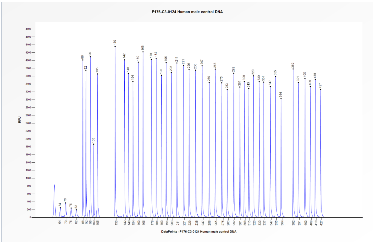
Figure 1. Capillary electrophoresis pattern from a sample of approximately 50 ng human male control DNA analysed with SALSA MLPA Probemix P176 CAPN3 (C3-0124).
