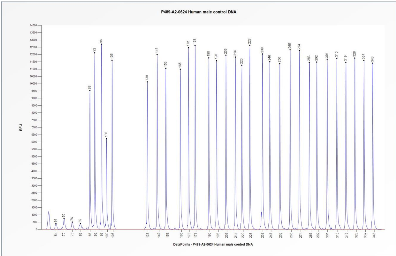
Figure 1. Capillary electrophoresis pattern from a sample of approximately 50 ng human male control DNA analysed with SALSA MLPA Probemix P489 BARD1 (A2-0624).
