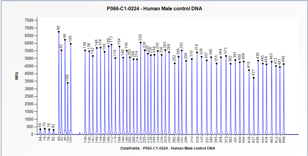
Figure 1. Capillary electrophoresis pattern from a sample of approximately 50 ng human male control DNA analysed with SALSA MLPA Probemix P066 Marfan Syndrome-2 (C1-0224).
