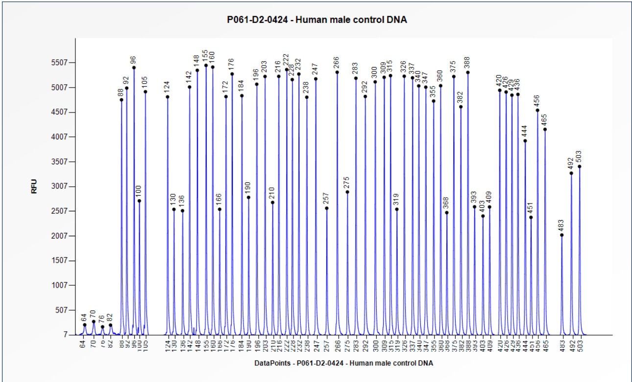
Figure 1. Capillary electrophoresis pattern from a sample of approximately 50 ng human male control DNA analysed with SALSA MLPA Probemix P061 Lissencephaly (D2-0424).
