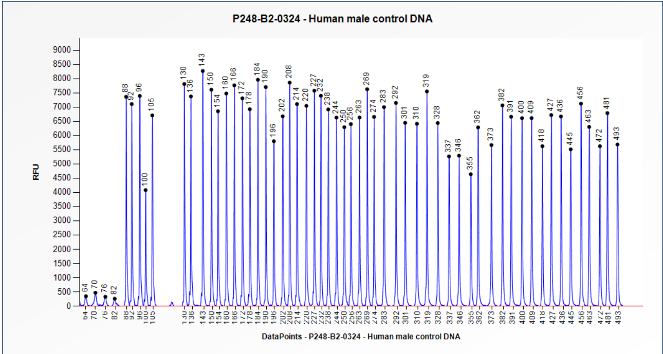
Figure 1. Capillary electrophoresis pattern from a sample of approximately 50 ng human male control DNA analysed with SALSA MLPA Probemix P248 MLH1-MSH2 Confirmation (B2-0324).
