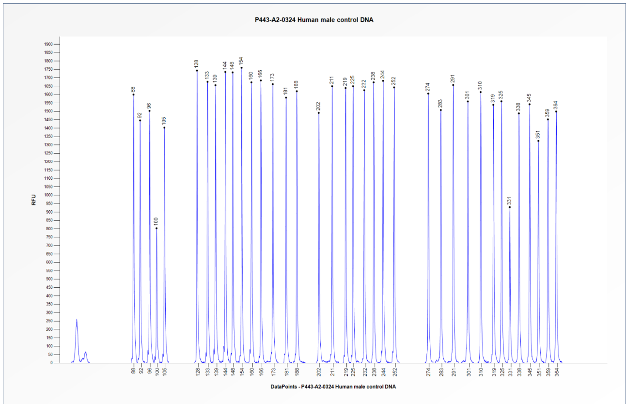
Figure 1. Capillary electrophoresis pattern from a sample of approximately 50 ng human male control DNA analysed with SALSA MLPA Probemix P443 KANSL1 (A2-0324).
