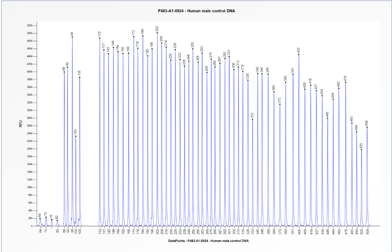
Figure 1. Capillary electrophoresis pattern from a sample of approximately 50 ng human male control DNA analysed with SALSA MLPA Probemix P483 HER gene family (A1-0924).
