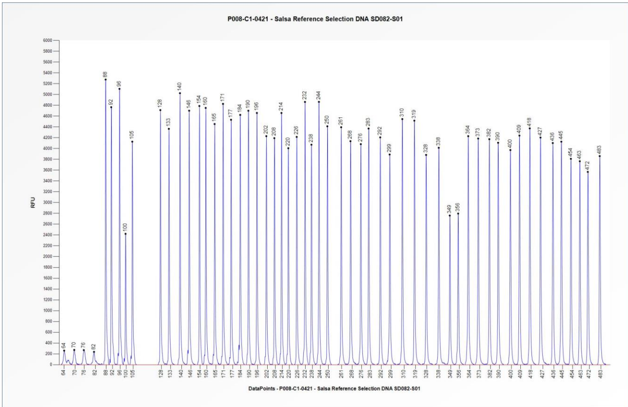
Figure 1. Capillary electrophoresis pattern from SALSA Reference Selection DNA SD082-S01 (approximately 50 ng) analysed with SALSA MLPA Probemix P008 PMS2 (C1-0421). Reference Selection DNA SD082 has two copies for each of the ten SNP probe targets present in P008 PMS2.
