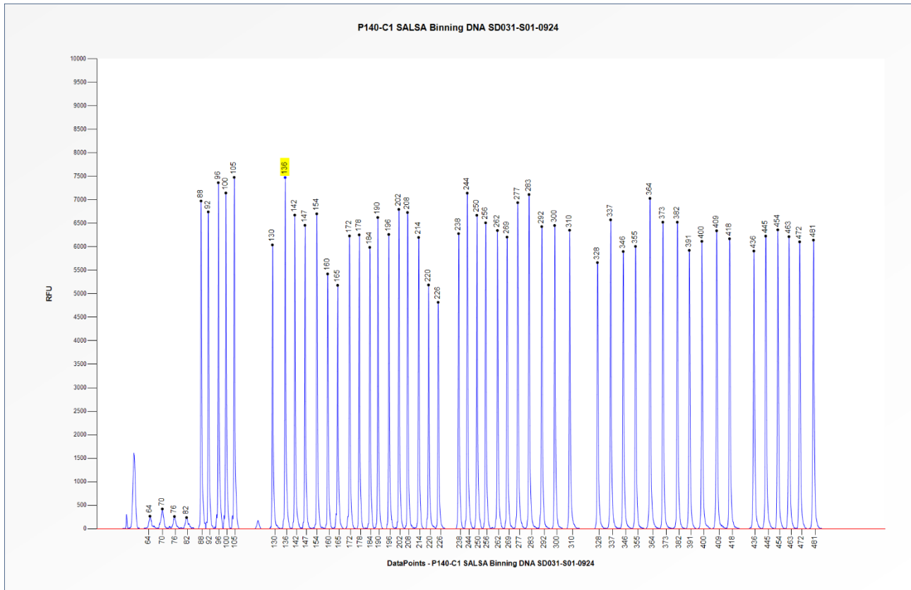
Figure 1. Capillary electrophoresis pattern from SALSA Binning DNA SD031-S01-0924 (approximately 50 ng) analysed with SALSA MLPA Probemix P140 HBA (C1-0322). The location of the Hb Contant Spring mutation (HBA2:c.427T>C, p.*143Glnext*31) specific probe at 136 nt is indicated. Probe peak heights may vary between different lots of the P140-C1 probemix.
