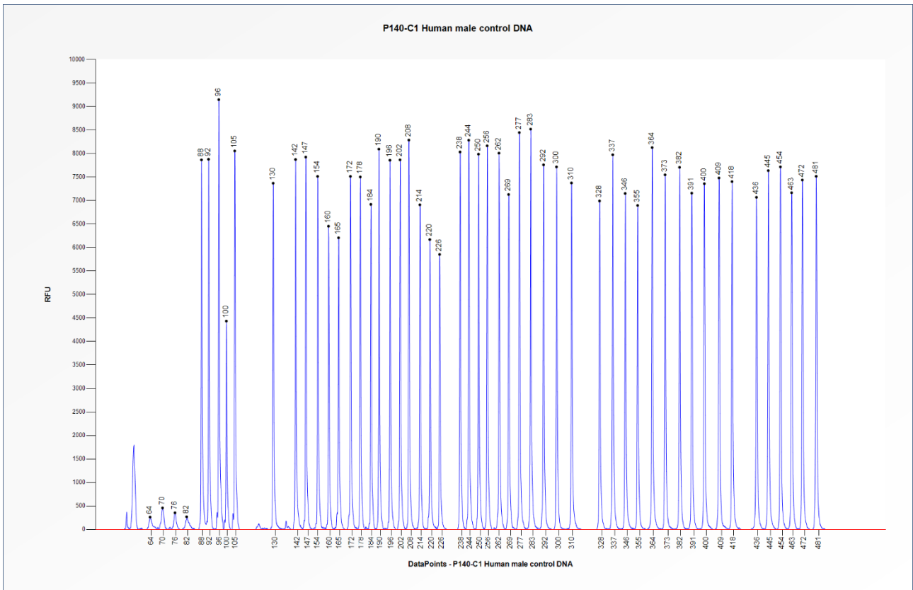
Figure 2. Capillary electrophoresis pattern from a sample of approximately 50 ng human male control DNA analysed with SALSA MLPA Probemix P140 HBA (C1-0322). Probe peak heights may vary between different lots of the P140-C1 probemix.
