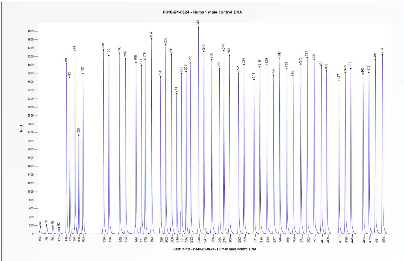
Figure 1. Capillary electrophoresis pattern from a sample of approximately 50 ng human male control DNA analysed with SALSA MLPA Probemix P340 EHMT1 (B1-0624).
