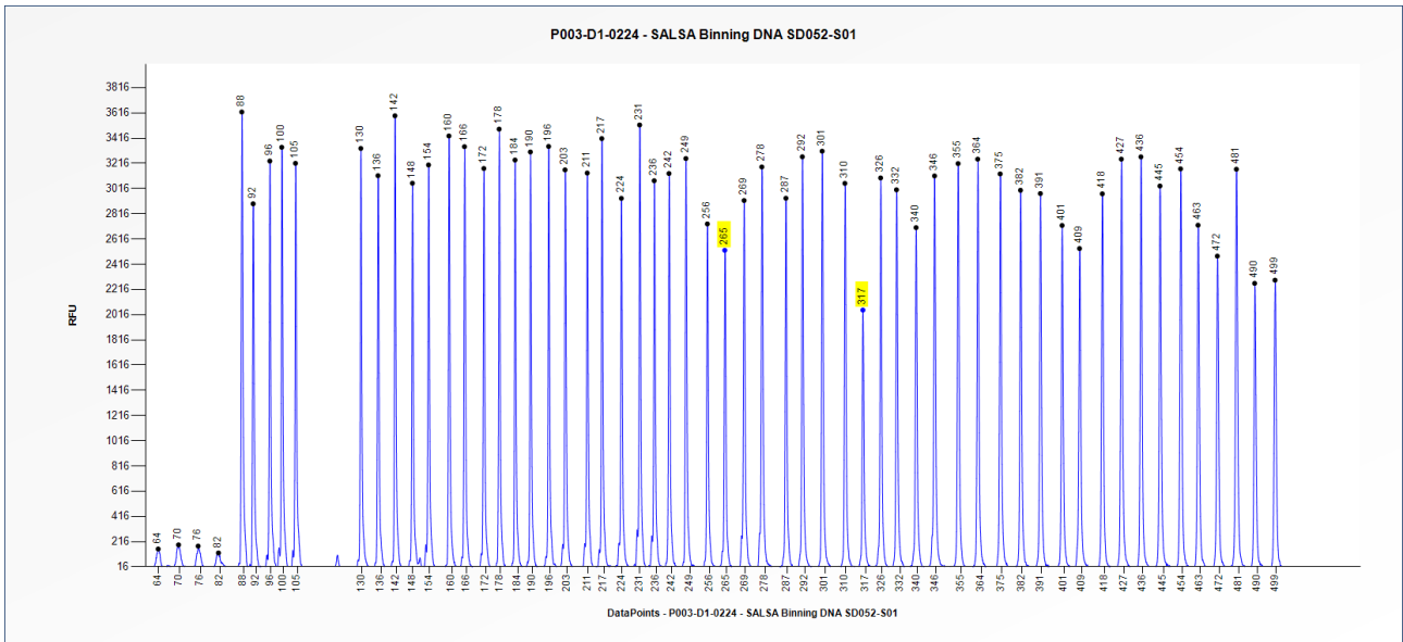
Figure 2. Capillary electrophoresis pattern from SALSA Binning DNA SD052-S01 (approximately 50 ng) analysed with SALSA MLPA Probemix P003 MLH1/MSH2 (D1-0224). The locations of the MSH2 10 Mb inversion specific probes at 265 and 317 nt are indicated.
