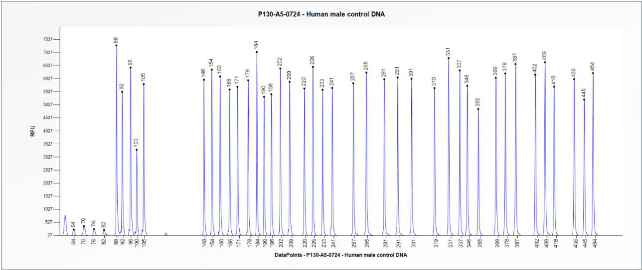
Figure 1. Capillary electrophoresis pattern from a sample of approximately 50 ng human male control DNA analysed with SALSA MLPA Probemix P130 CCM Mix-1 (A5-0724).
