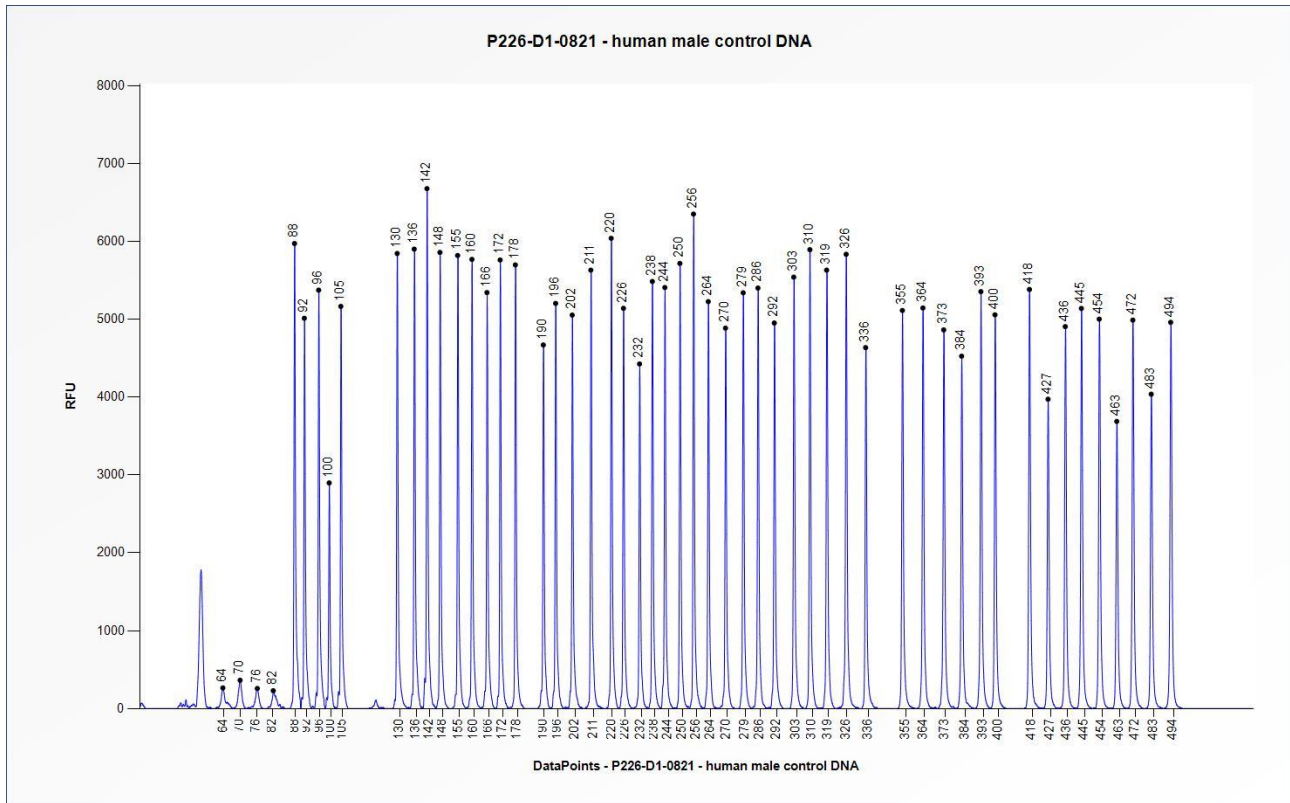
Figure 1. Capillary electrophoresis pattern from a sample of approximately 50 ng human male control DNA analysed with SALSA MLPA Probemix P226 SDH (D1-0821).
