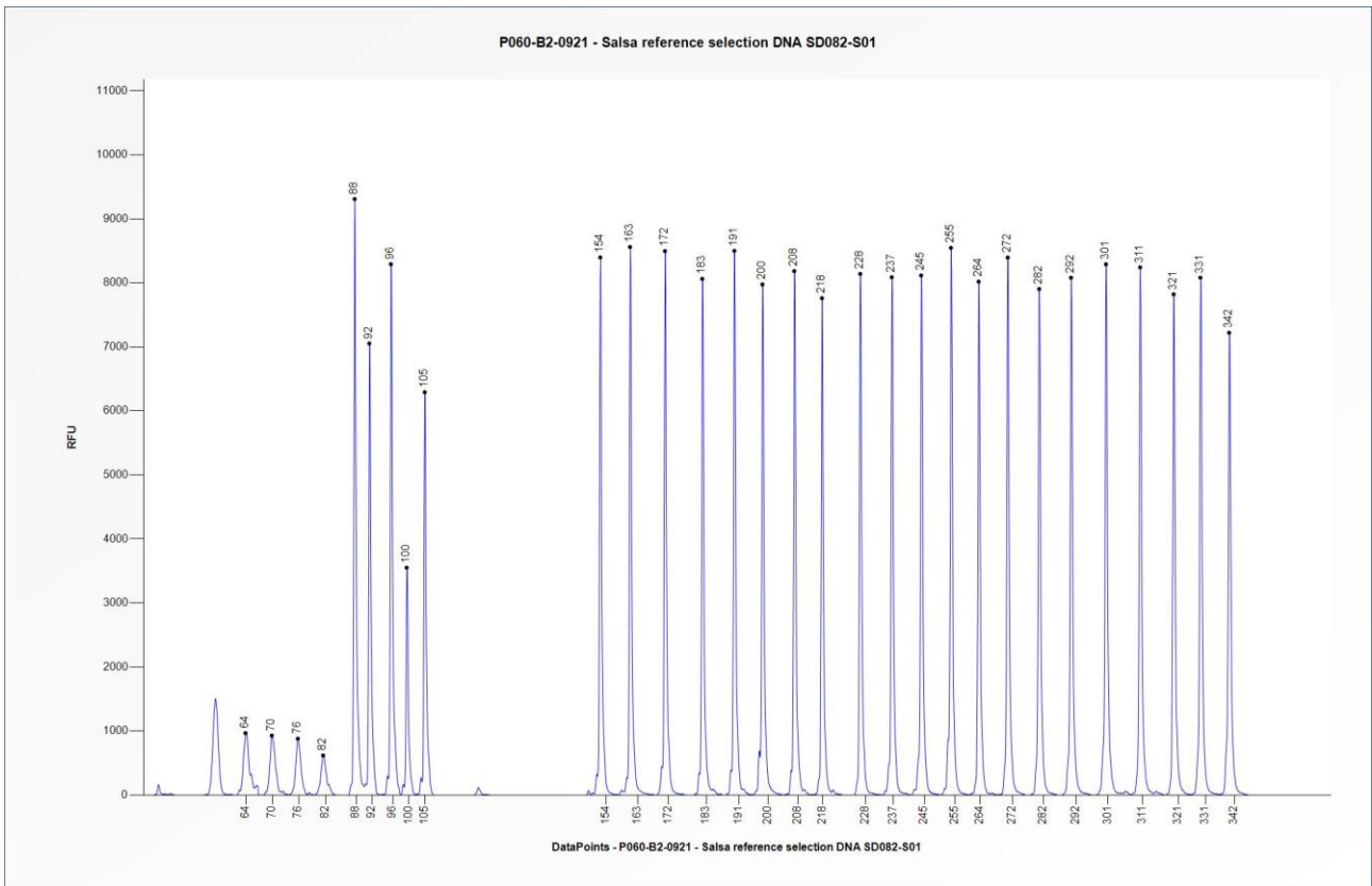
Figure 2. Capillary electrophoresis pattern from SALSA Reference Selection DNA SD082-S01 (approximately 50 ng) analysed with SALSA MLPA Probemix P060 SMA Carrier (B2-0921).
