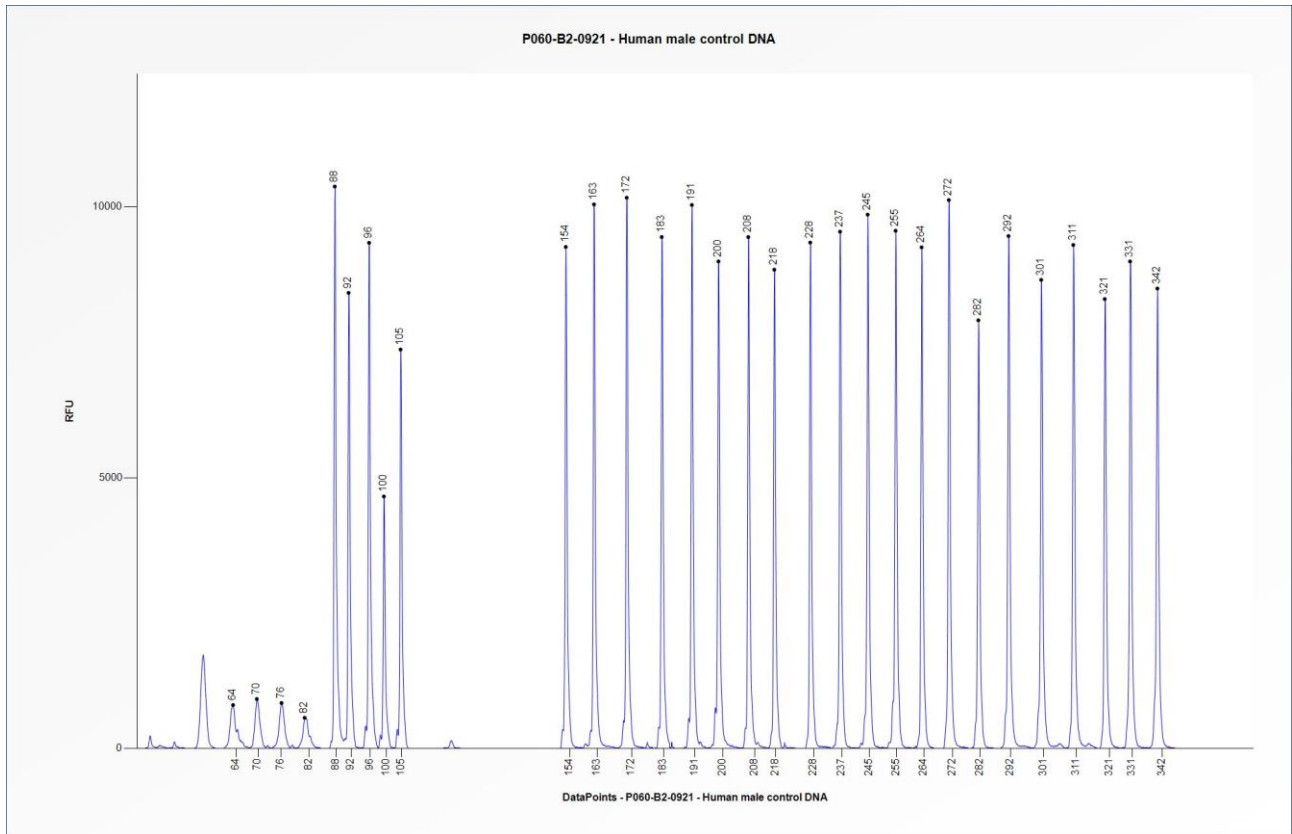
Figure 1. Capillary electrophoresis pattern from a sample of approximately 50 ng human male control DNA analysed with SALSA MLPA Probemix P060 SMA Carrier (B2-0921).
