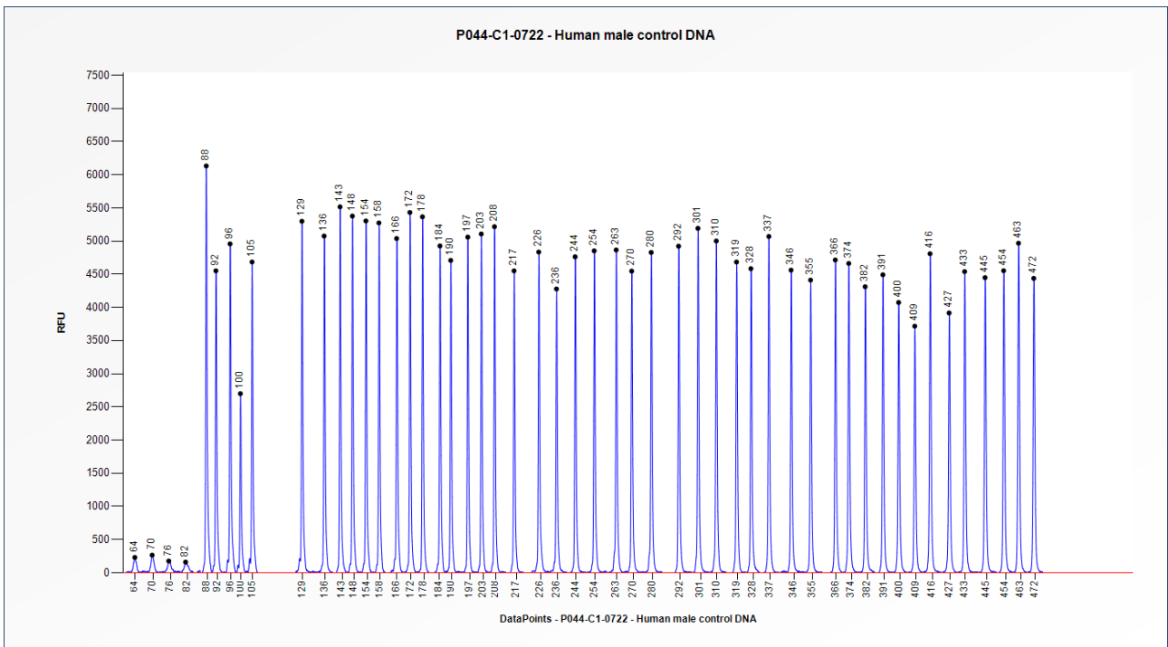
Figure 1. Capillary electrophoresis pattern from a sample of approximately 50 ng human male control DNA analysed with SALSA MLPA Probemix P044 NF2 (C1-0722).
