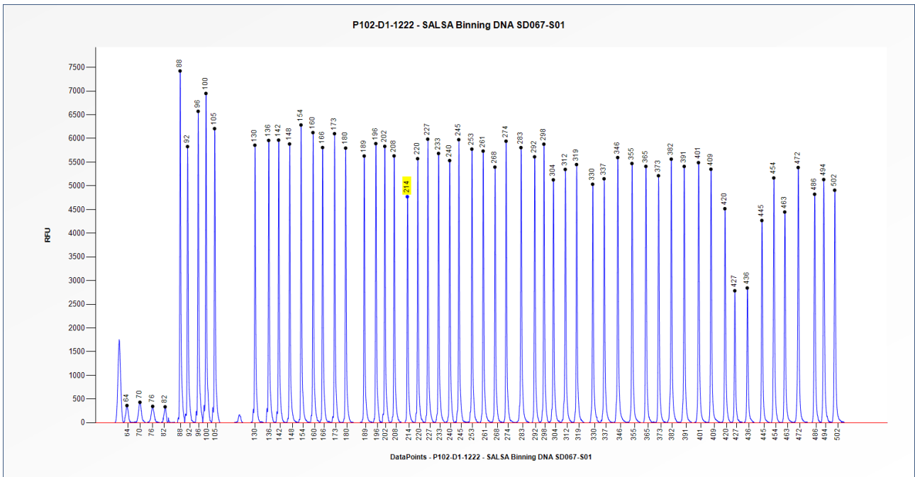
Figure 2. Capillary electrophoresis pattern from SALSA Binning DNA SD067-S01 (approximately 50 ng) analysed with SALSA MLPA Probemix P102 HBB (D1-1222). The location of the haemoglobin S mutation-specific probe at 214 nt is indicated.
