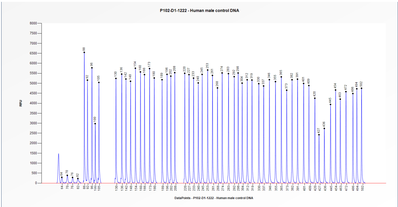
Figure 1. Capillary electrophoresis pattern from a sample of approximately 50 ng human male control DNA analysed with SALSA MLPA Probemix P102 HBB (D1-1222).
