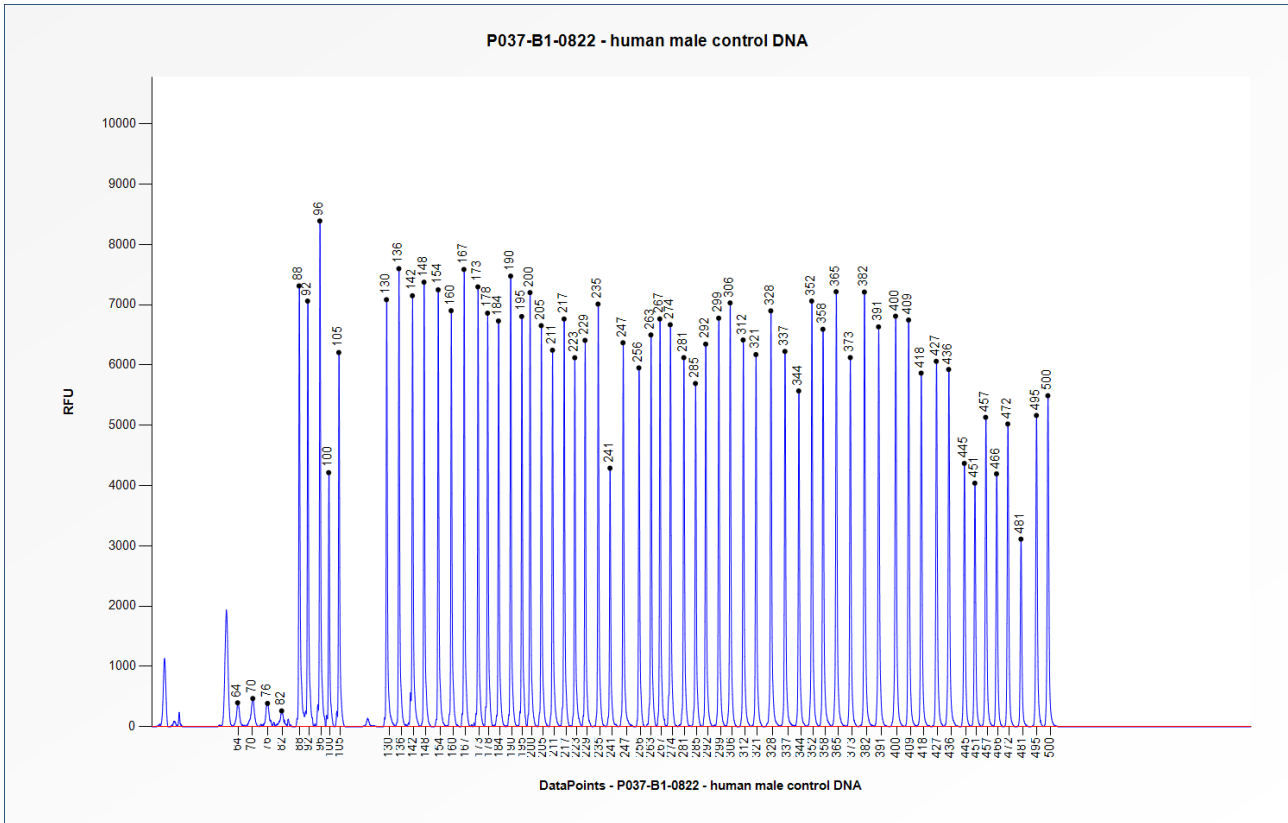
Figure 1. Capillary electrophoresis pattern from a sample of approximately 50 ng human male control DNA analysed with SALSA MLPA Probemix P037 CLL-1 (B1-0822).
